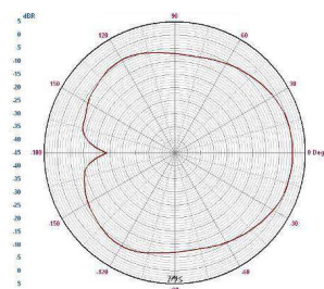
Fig. 2. Cardioid pattern
