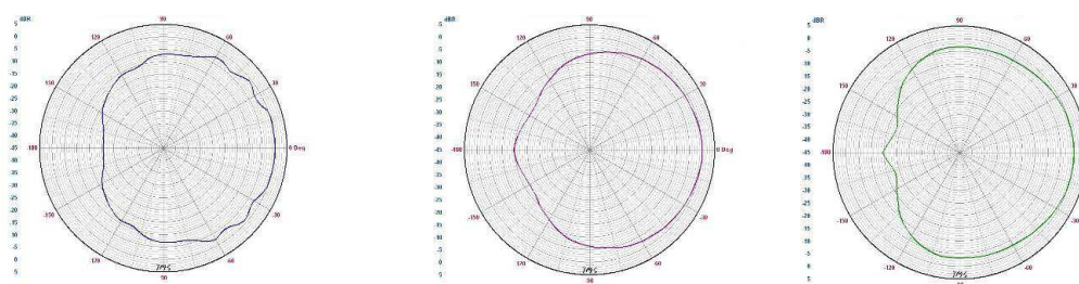
Fig. 6. Back energy rejection at 40 Hz / 50 Hz / 63 Hz
