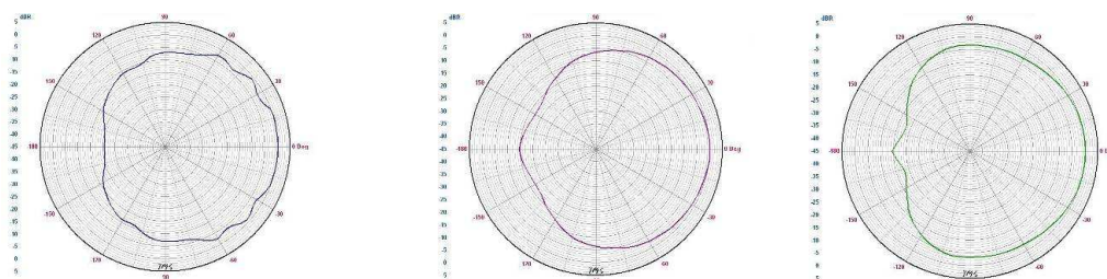
Fig.9. Back energy rejection at 40 Hz / 50 Hz / 63 Hz
