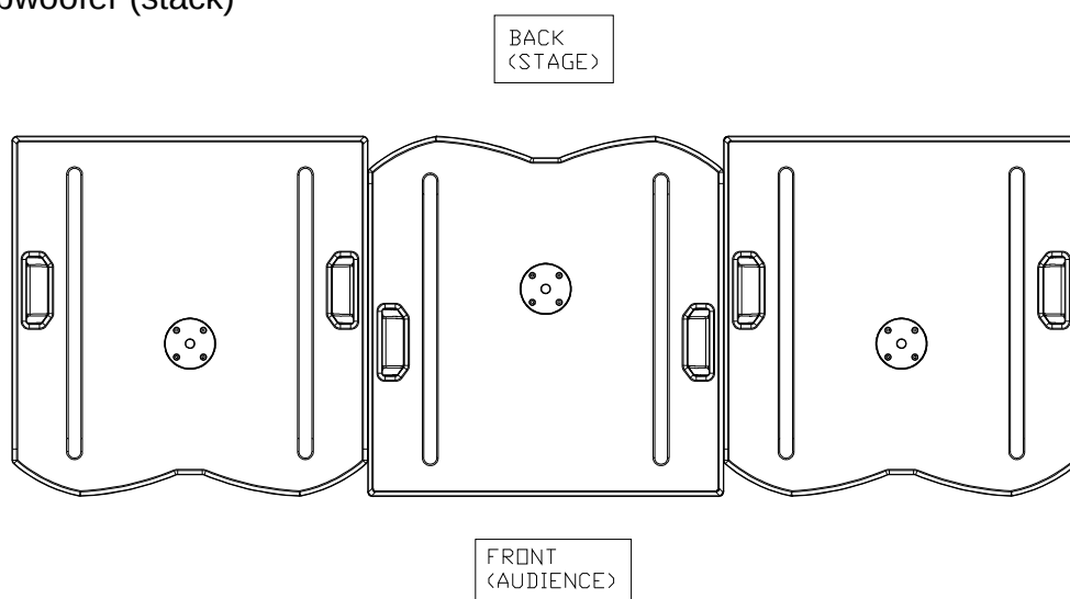
Fig. 7. Cardioid configuration for XW118 (horizontal line)
