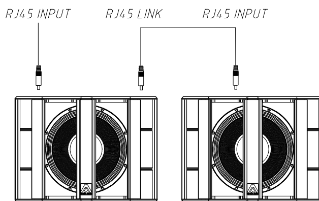
Fig.12. Parallel connection for the XW118 (network). You can link up to eight units when using DANTE networking, or more when not using it.
