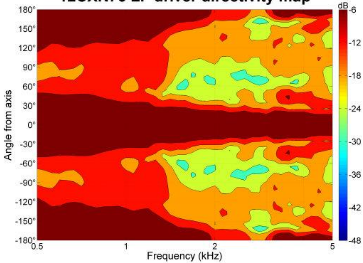
12CXN76 LF driver directivity map
