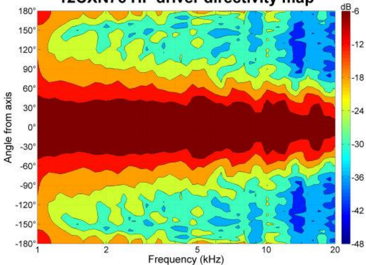
12CXN76 HF driver directivity map
