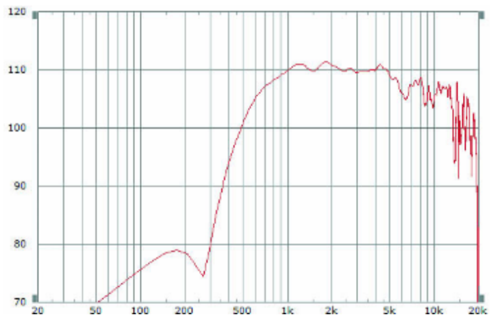
Sensitivity B&C DE920 1W 1m
