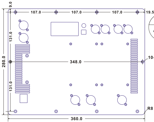
Installation dimension drawing (Unit: mm)
