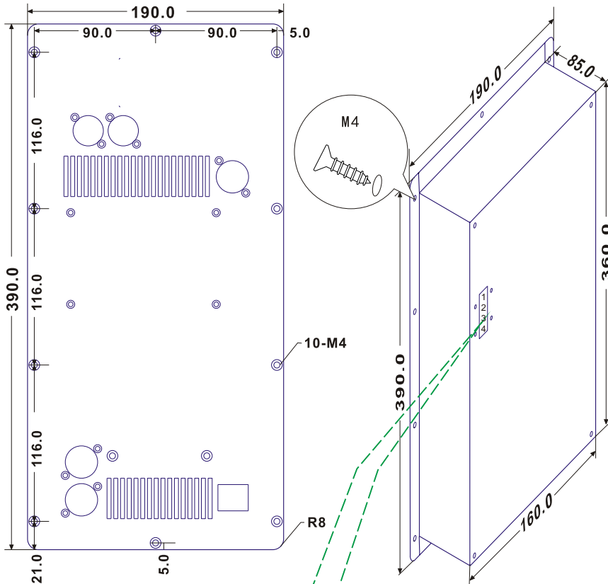
Installation dimension drawing (Unit: mm)
