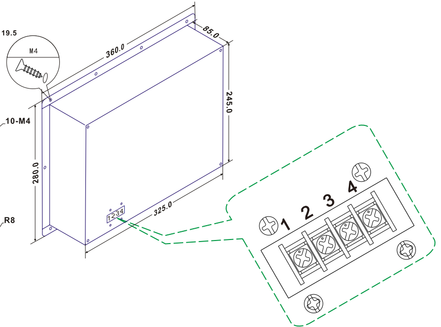
Installation dimension drawing (Unit: mm)
