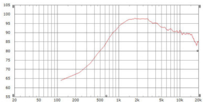
Sensitivity unsmoothed 2,83V 40hm 1m
