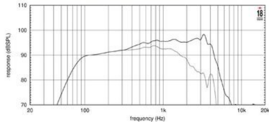
FREQUENCY RESPONSE MADE IN 25 L.T. ENCLOSURE TUNED AT 65 Hz IN FREE FIELD (4th) ENVIRONMENT. ENCLOSURE CLOSES THE REAR OF THE DRIVER, THE THIN LINE REPRESENTS 45° OFF AXIS FREQUENCY RESPONSE
