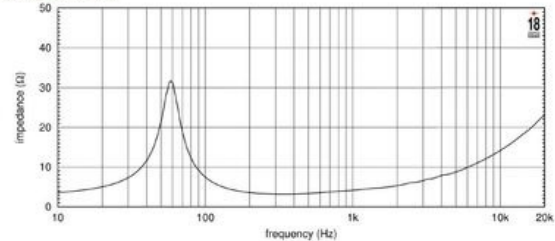
FREE AIR IMPEDANCE CURVE
